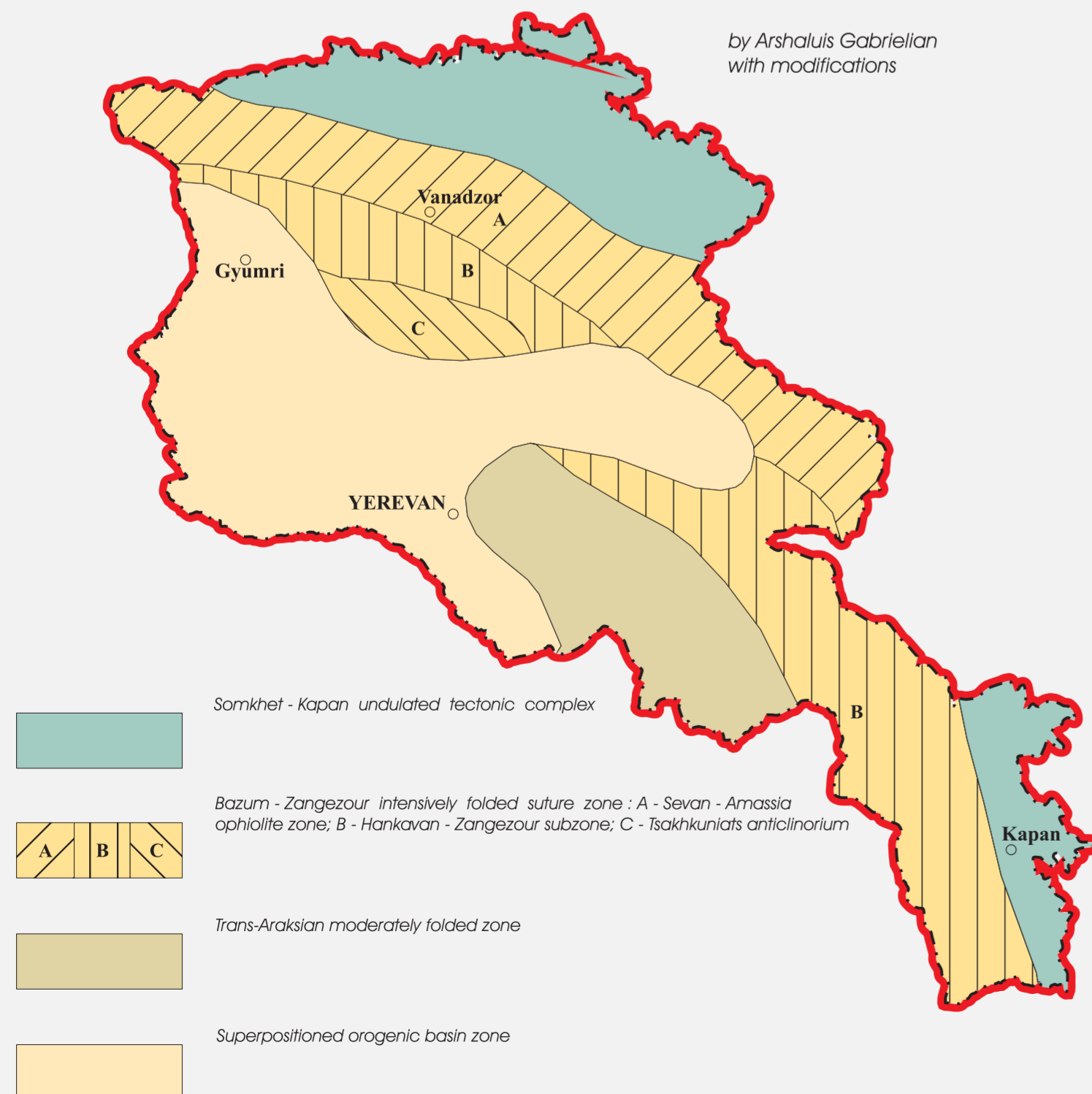
Geotectonic zonation scheme of the Republic of Armenia Scale 1:1 500 000
